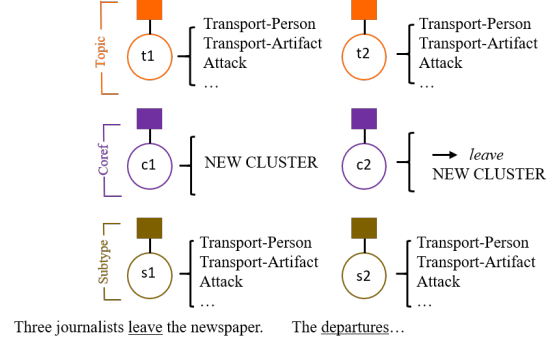
Figure 1: Unary factors for the three tasks, the variables they are connected to, and the possible values of the variables.
