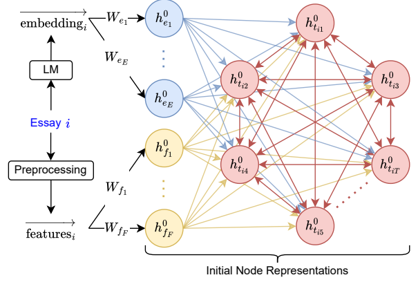
Figure 1: Constructing the graph from an input essay.
